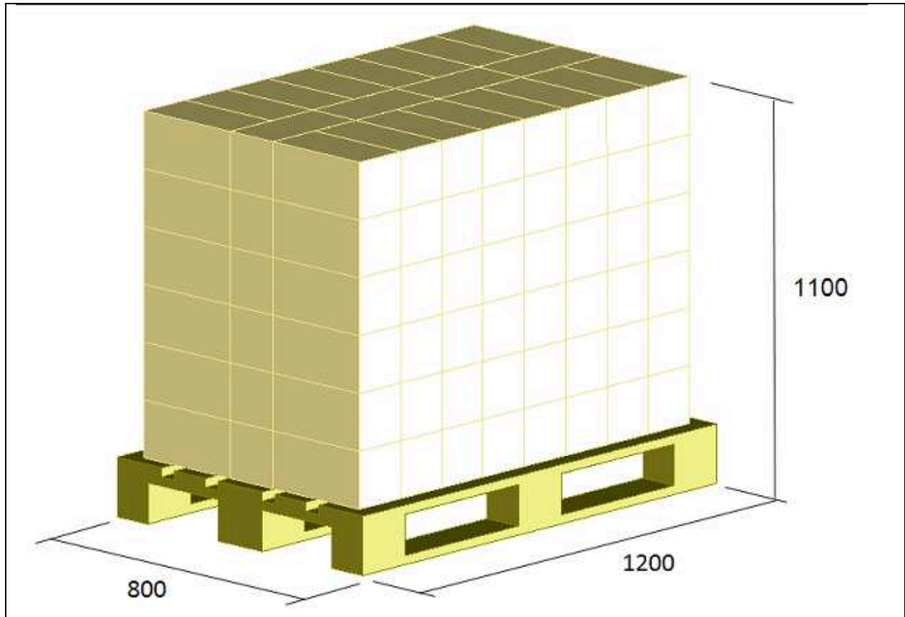
Figure 6 – Pallet Stacking Layout
