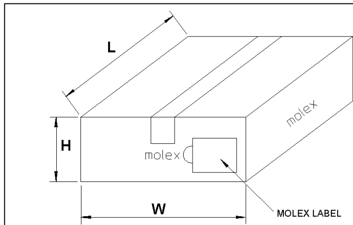
Figure 4: Box dimensions
